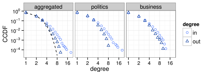
Fig. 1. Distribution of degrees for the aggregated network and the subnetworks that are induced by article feeds, given as the complementary cumulative degree distribution P[d \geq d_x] . The degrees of nodes in subnetworks include edges to and from nodes of different types. The dashed line represents the expected distribution for an Erdős-Rényi graph of the same size.
