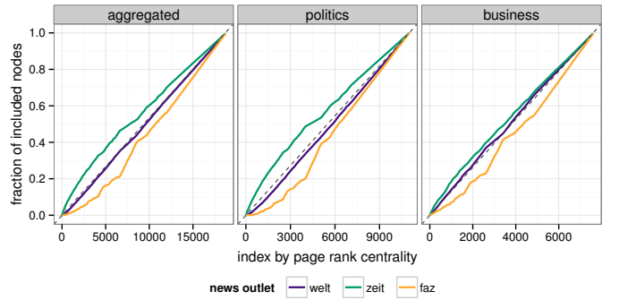
Fig. 4. Fraction of articles by news outlet that are included among the k highest ranked articles by PageRank centrality. The index k is increased by steps of 100 and all values are averaged over 100 runs to account for ties in the ranking. The dashed line denotes the performance of a random ranking.
