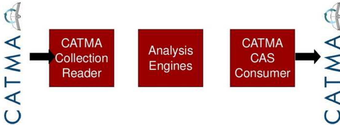
Figure 1: End-To-End architecture of combining the collaborative annotation platform CATMA with the automatic text processing pipeline UIMA.
